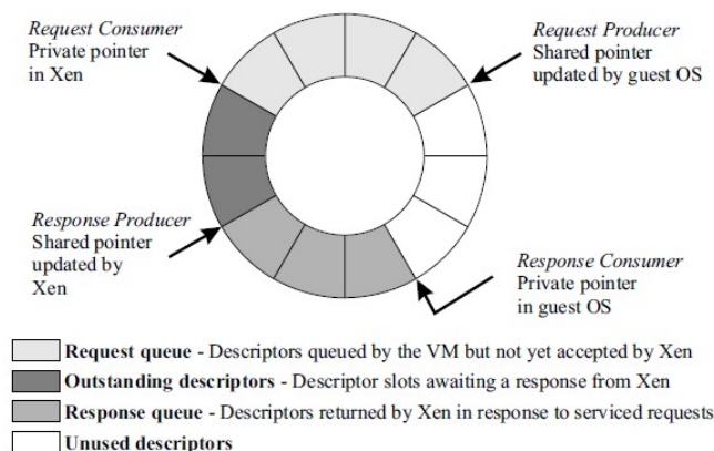
Fig. 1. The structure of asynchronous I/O rings
