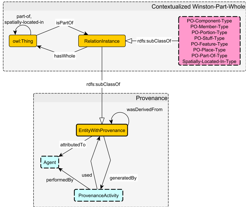
Figure 3. Schema Diagram for the Contextualized Winston Part-Whole Pattern extended by a Provenance pattern following PROV-O.
