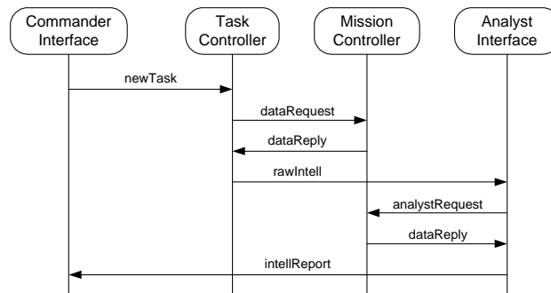
Fig. 3. Sequence Diagram
