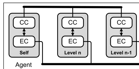
Figure 1: OBAA++ agent architecture
