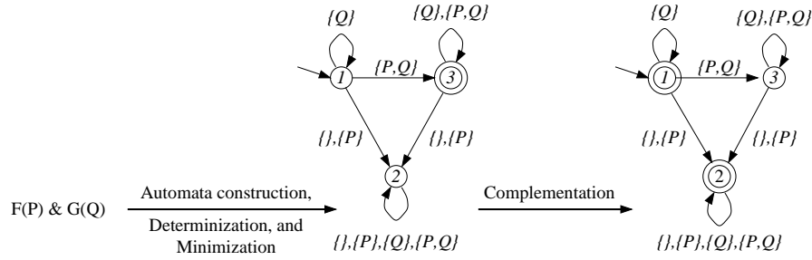
Fig. 10. A formula and the corresponding automata
