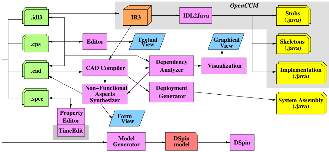
Figure 4: Cadena architecture
