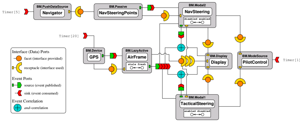
Figure 1: Simple avionics system
